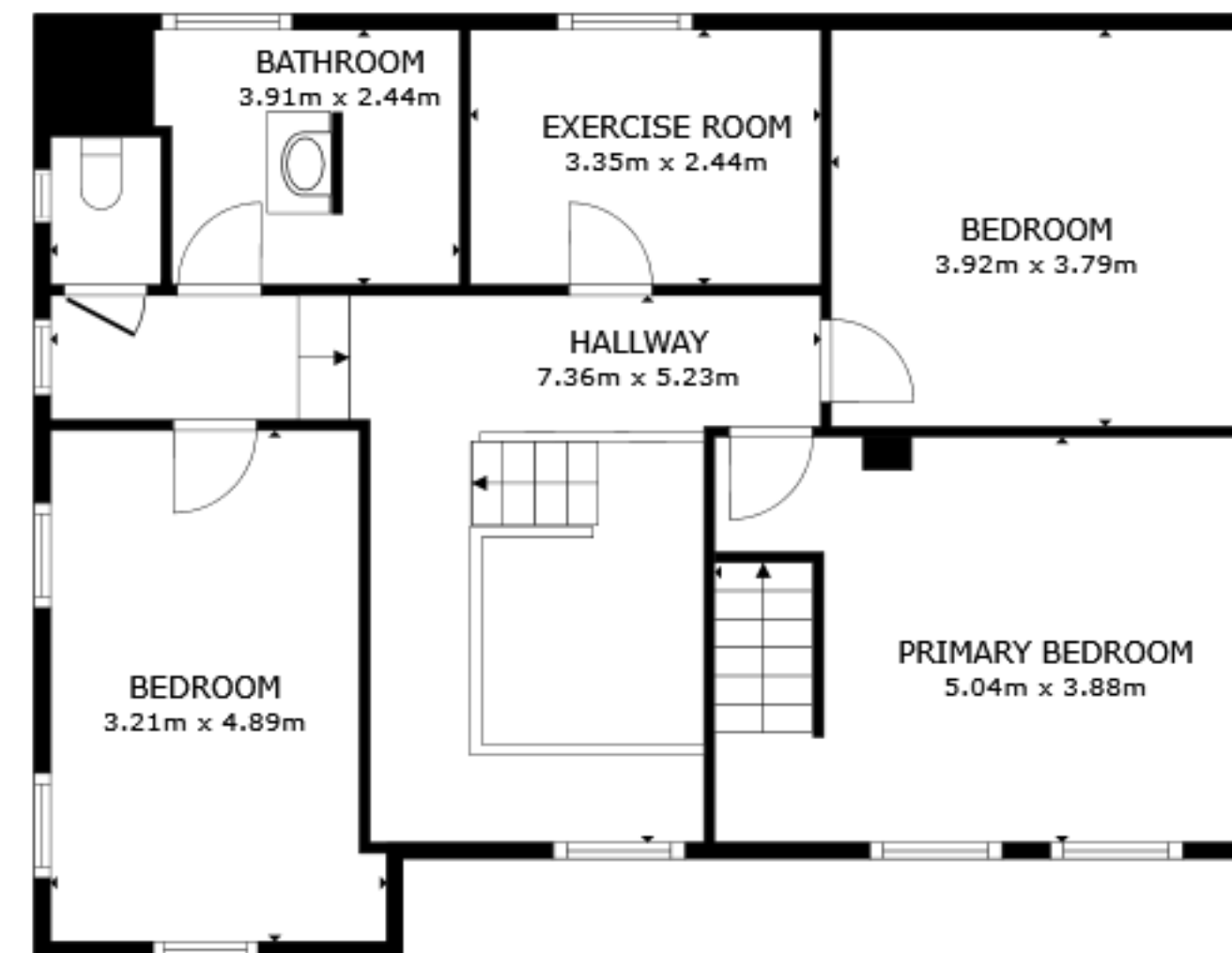
FLOOR 2
