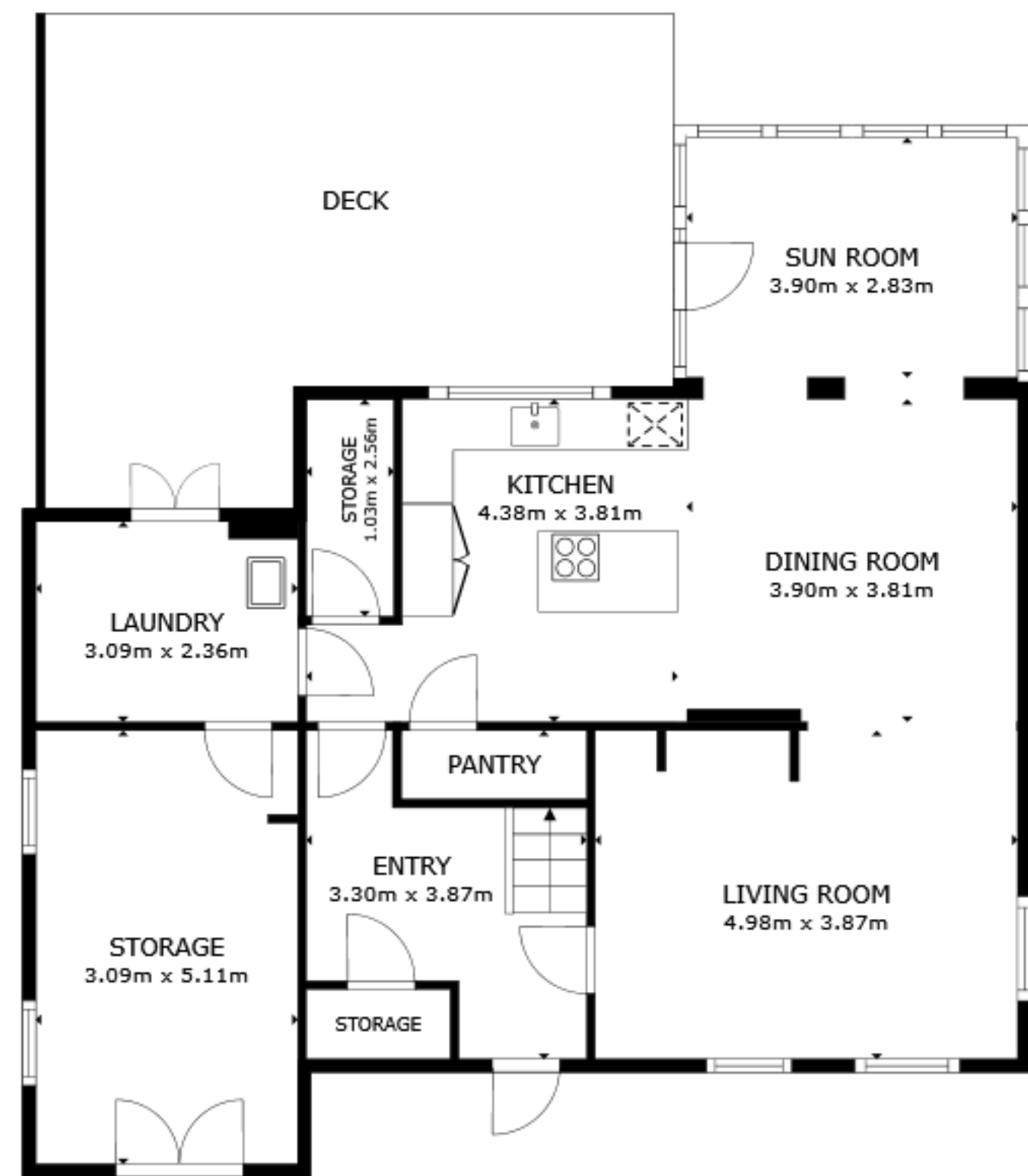
FLOOR 1
